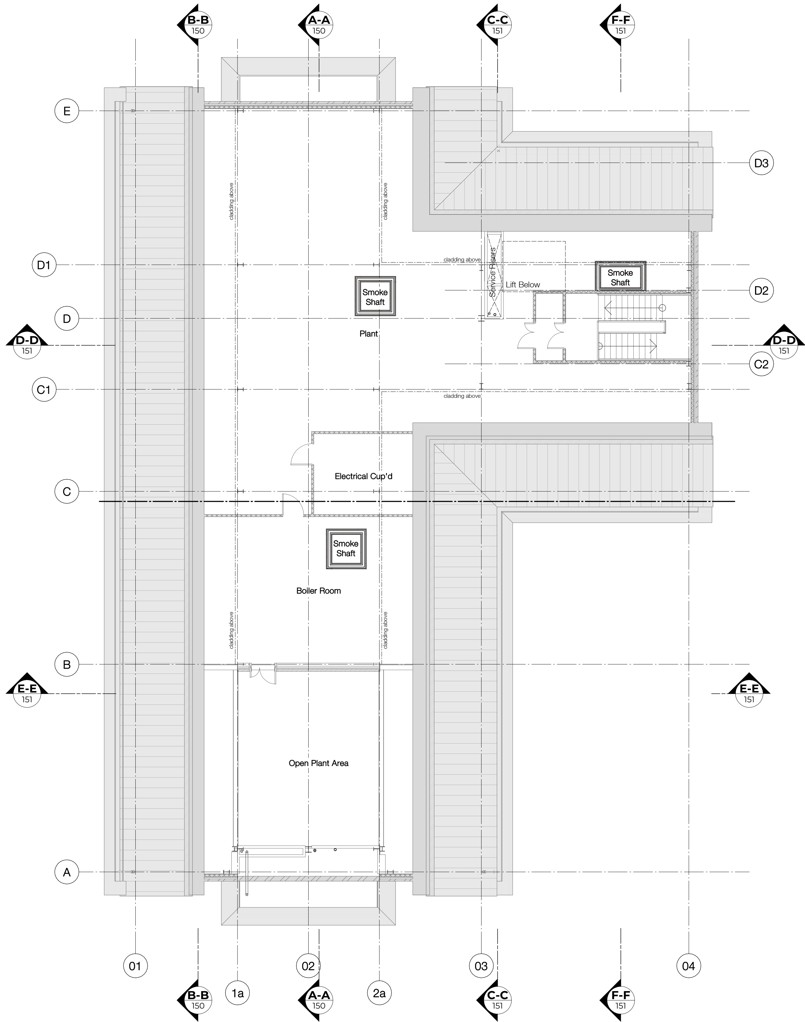
PROPOSED THIRD GA PLAN SCALE 1 : 100
