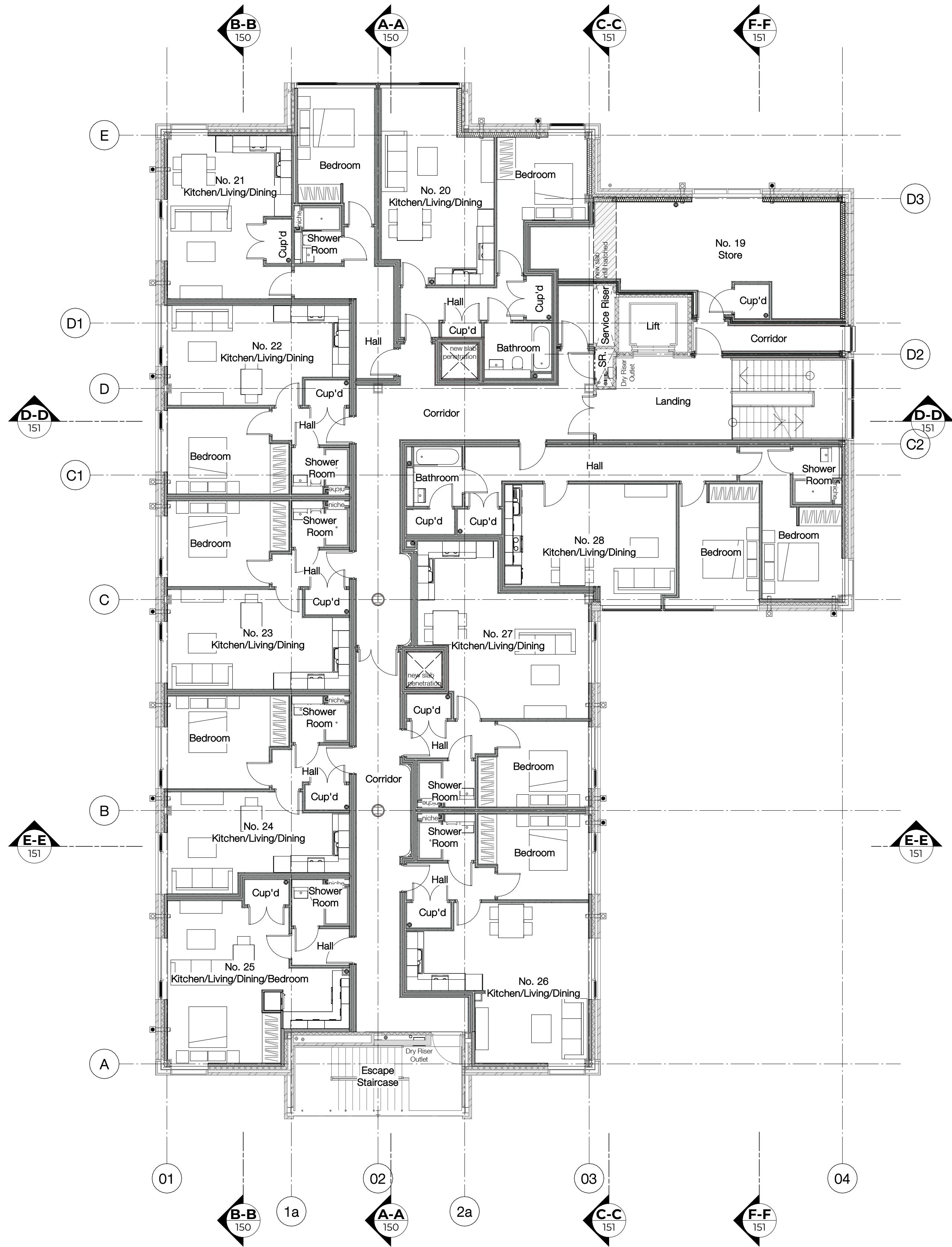
PROPOSED SECOND GA PLAN SCALE 1 : 100
